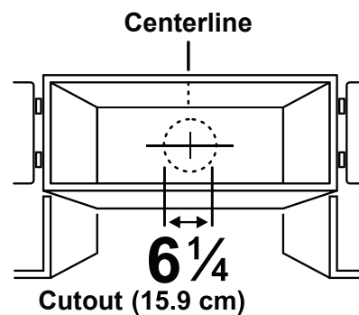
Wall/Side Cutout (B)
