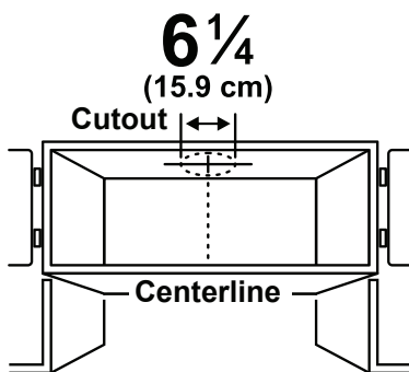
Cabinet Top Cutout (A)
